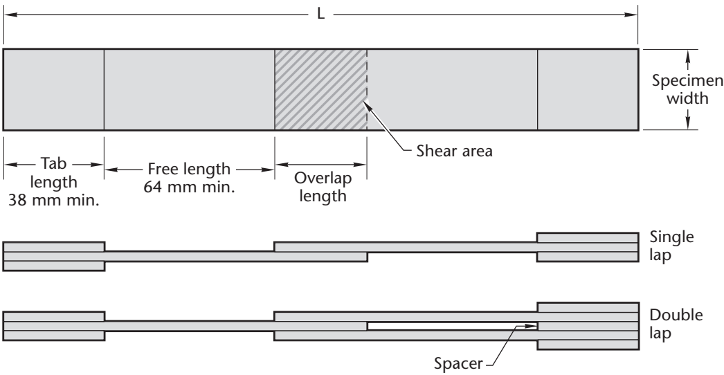
Figure Q1 Overlap Tension Specimen (See Clauses Q4 and Q6.4.)
